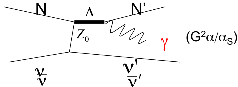
Radiative Delta Decay
