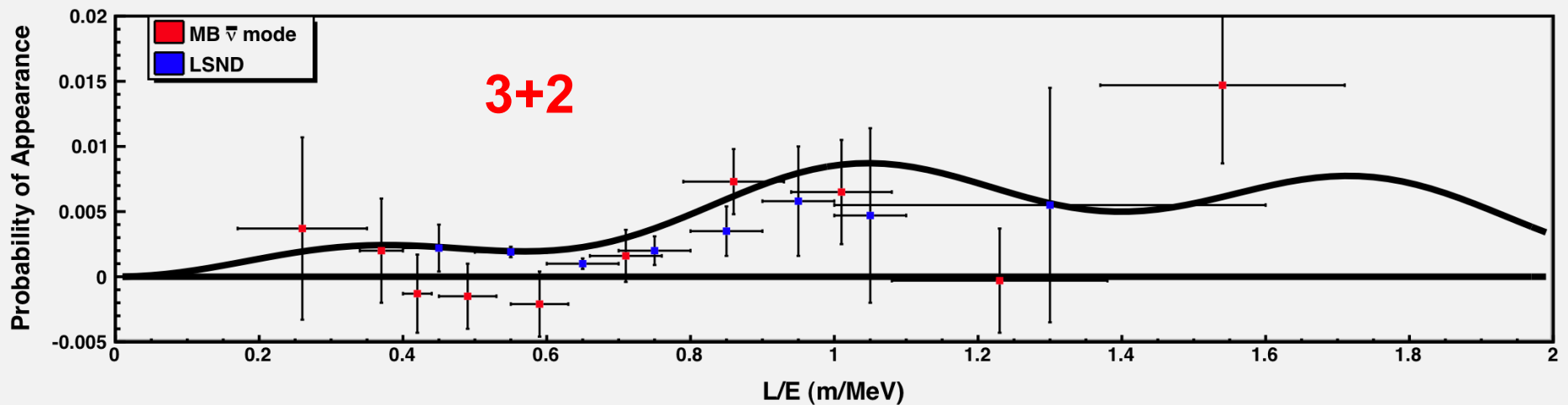
(3+2) Vb \bar{\nu}_\mu Model Antineutrino Appearance
