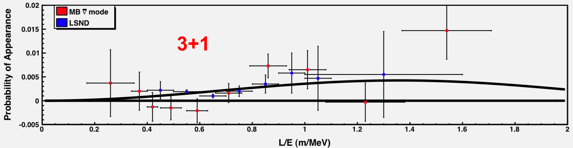
(3+1) \bar{\nu}_\mu Model Antineutrino Appearance
